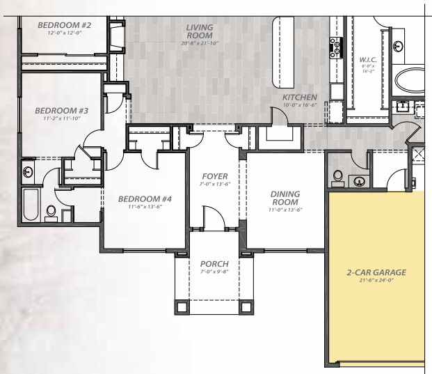
Floor Plan with Option D Bedroom #4 and Dining Room added
